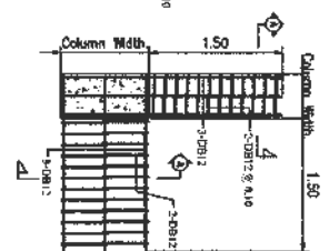
Reinf. For Shear Stirrup Type 'C'
