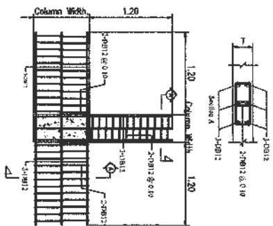
Reinf. For Shear Stirrup Type 'B'
